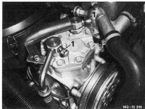
York refrigerant compressor Engine 110
